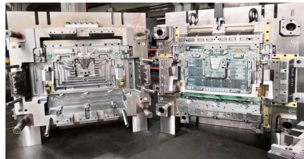
Auto Part - Roof system frame
